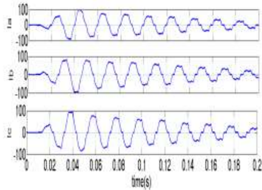
Fig-8: Current waveform
