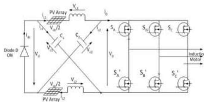
Fig. 2: EZ-source inverter circuit
