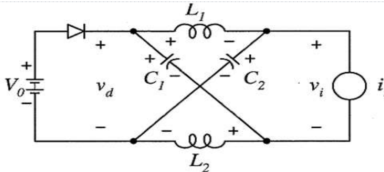
Fig-1: Z-Source inverter circuit
